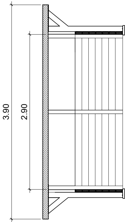
Dimensions (m)
